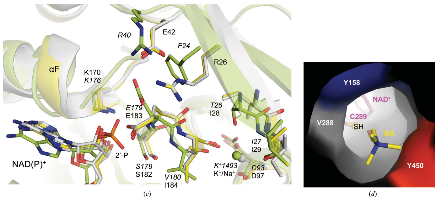
Figure 7 (continued) (c) Local structural features/changes that may favor binding of the 2'-P group of NADP + in PaBADH (light green) and impede binding in SaBADH [NAD– SaBADH BME(+) , yellow; NAD– SaBADH BME(-) , light gray]. The presence of Ile28 ( SaBADH ) instead of the equivalent Thr26 ( PaBADH ) may change the coordination geometry of a metal (shown as spheres; K + 1493, light green, PaBADH ; Na + /K + , light gray, SaBADH ; see Figs. 6 d and 6 e ) and thus possibly affect the lower affinity of SaBADH for NADP + . (d) Merged model based on multiple structural superposition showing NAD + and Cys289 from NAD–G234S- SaBADH BME(-) and residues Val288 (gray), Tyr158 (blue) and Tyr450 (red) from apo SaBADH BME(+) PEG and betaine aldehyde (BA; carbon, yellow; nitrogen, blue; oxygen, red) from human mitochondrial ALDH.
